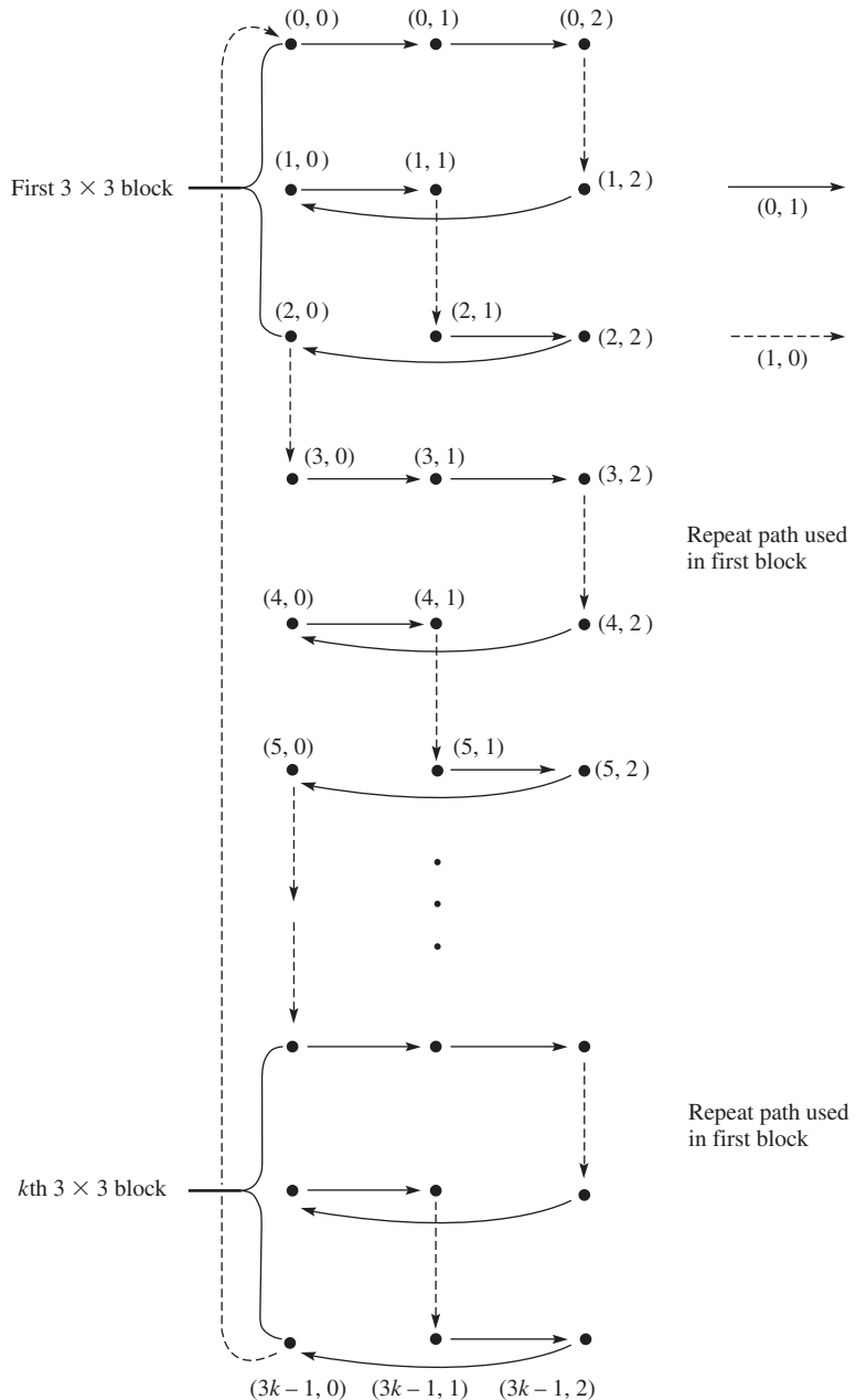
Figure 30.6 \text{Cay}(\{(1, 0), (0, 1)\}; \mathbb{Z}_m \oplus \mathbb{Z}_n) .
