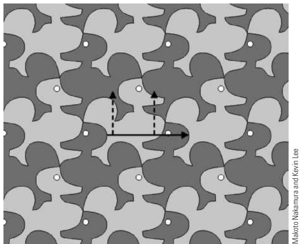
Figure 28.13 Fish5 by Makoto Nakamura, adapted by Kevin Lee. Design with symmetry group pg (disregarding shading). The solid arrow is the translation vector. The dashed arrows are the glide-reflection vectors.
