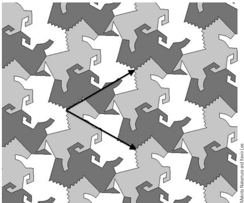
Figure 28.14 Horses1 by Makoto Nakamura, adapted by Kevin Lee. Design with symmetry group p3 (disregarding shading). The inserted arrows are translation vectors.
